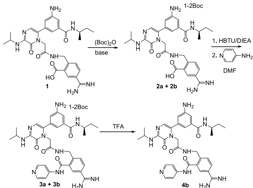
Scheme 1. Synthesis of compound 4b .
