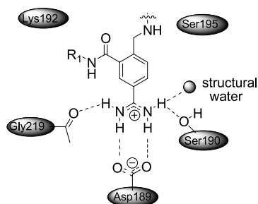
Figure 2. Schematic representation of the binding mode of the P 1 moiety of inhibitor with TF/VIIa complex.
