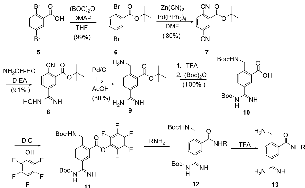
Scheme 2. Synthesis of P 1 side pocket analogs.
