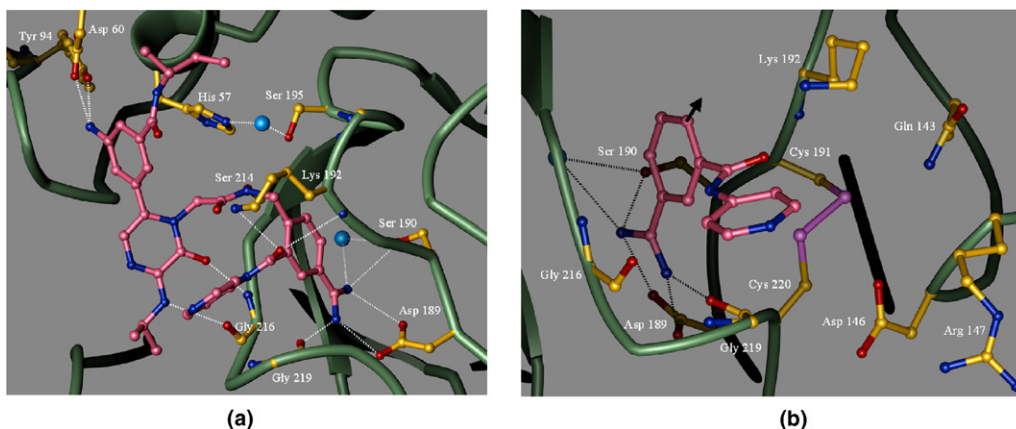
Figure 3. (a) Crystal structure of compound 4b bound in the active site of TF/VIIa complex. The structure has been refined to an R_{\text{free}} of 26.8% at 2.0 Å resolution ( R_{\text{crystal}} : 22.3%). Some of the key side chains of factor VIIa are displayed (C: gold, N: dark blue, O: red, and S: pink). The carbon atoms of the inhibitor are shown in dark pink color. The hydrogen bonds formed by the inhibitor are shown in dotted (white) lines. Two bound solvent molecules are shown as cyan spheres. One of them is bound near the active site serine and histidine side chains while the other solvent molecule (structural water) is bound in the S 1 pocket (b) close-up view of the S 1 side pocket (multi-colored as shown in Fig. 3a ). This figure is rotated relative to Figure 3a to clarify the position of the S 1 side pocket. Also, for clarity, only the benzamidine and the pyridyl amide of the inhibitor are shown. The black arrow indicates the approximate directionality of the connection between the benzamidine moiety and the rest of the inhibitor. The hydrogen bonds are shown in black dotted lines.
