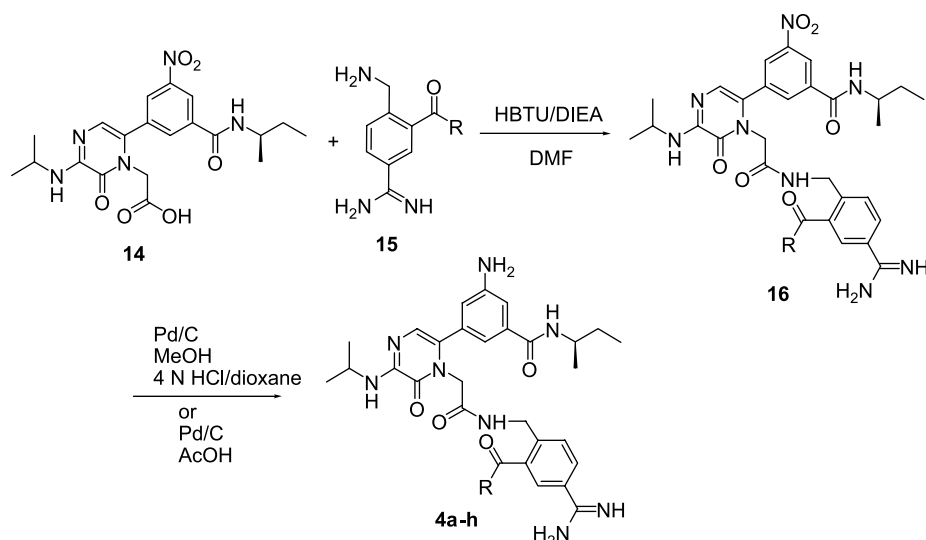
Scheme 3. Coupling of side pocket P 1 analogs to pyrazinone core.
